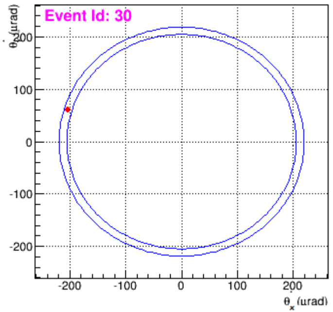
Angular Topology
