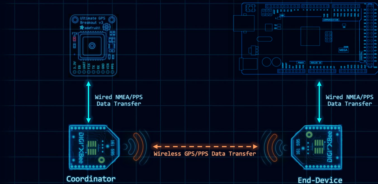
Figure 8.02 – Wireless GPS Data Relay Concept
