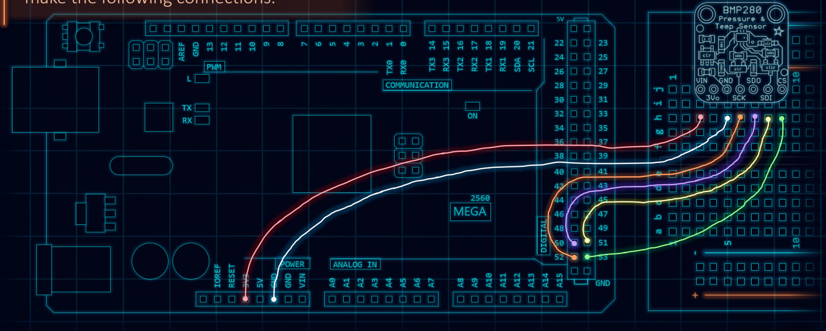
Figure 9.03 – Arduino ATmega2560 - BMP280 Sensor Wiring Setup
