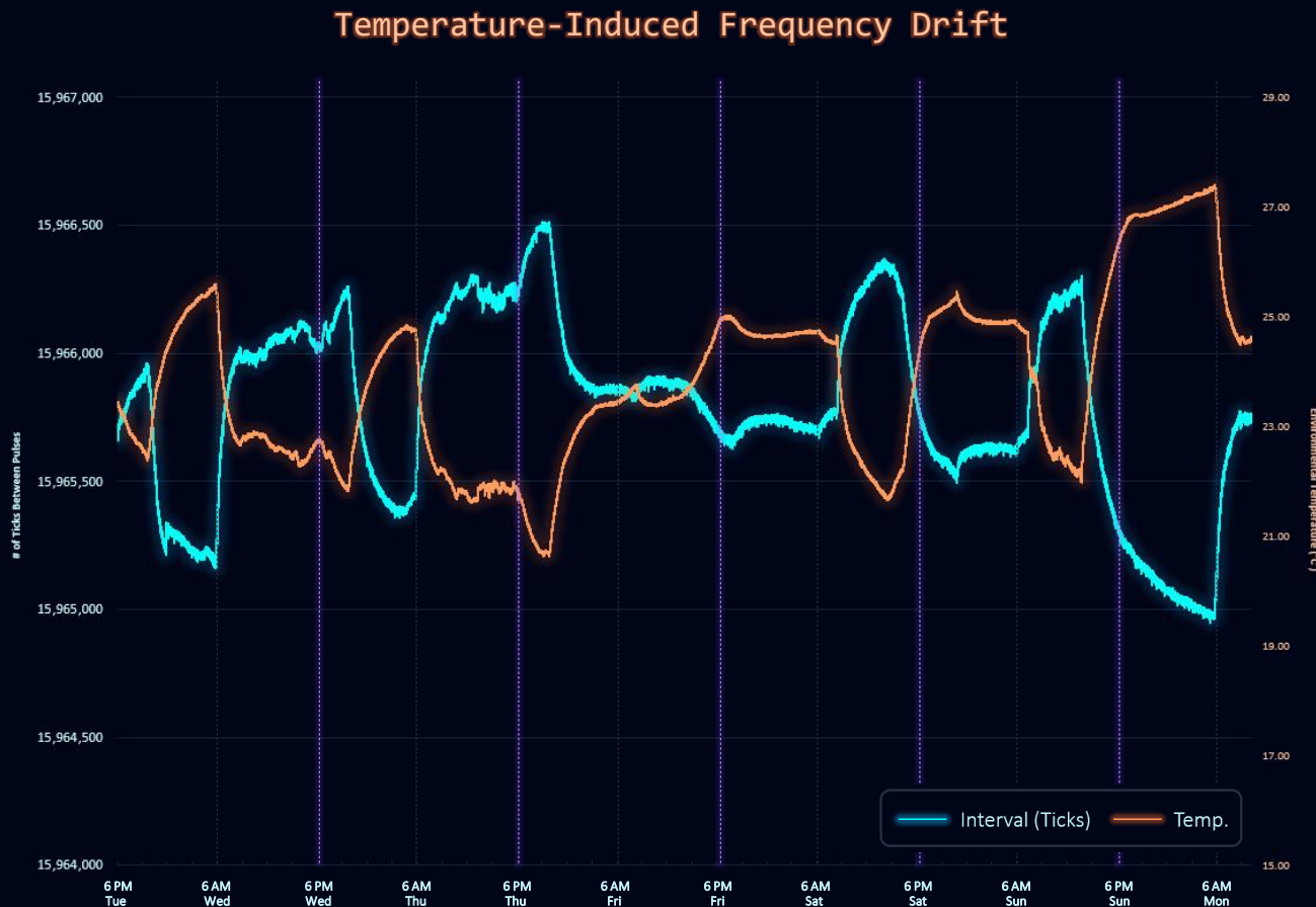
Figure 9.11 – Oscillator Drift Scatter Plot
