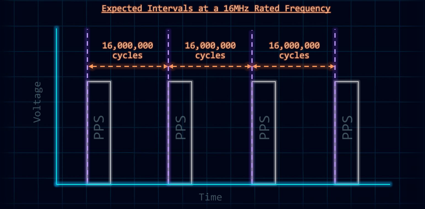
Figure 8.04 – PPS Signal with Expected Interval Timing
