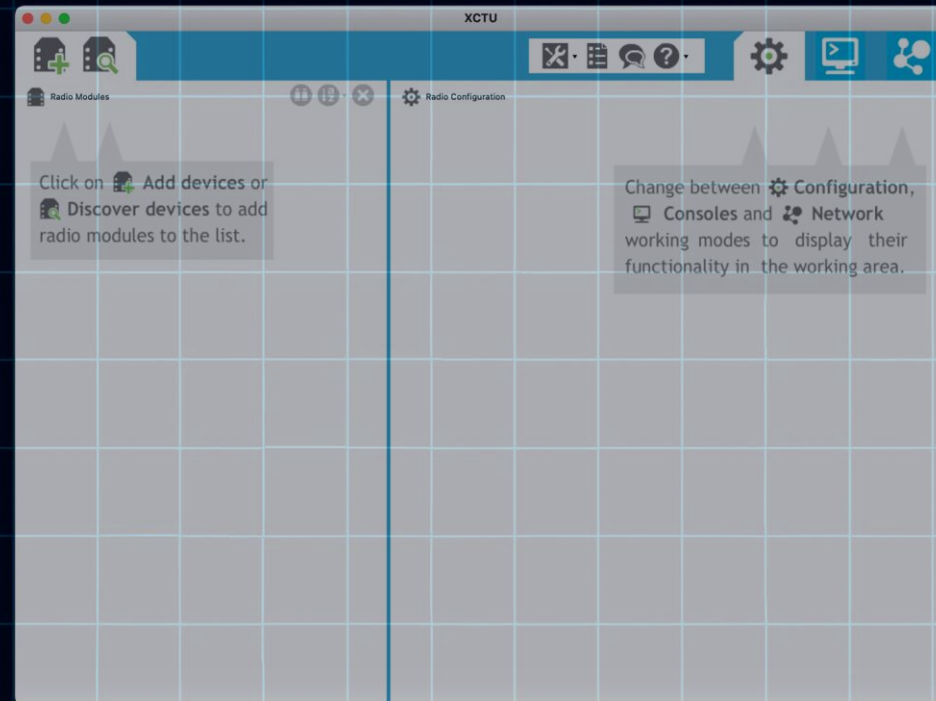
Figure 3.03 – XCTU Interface
