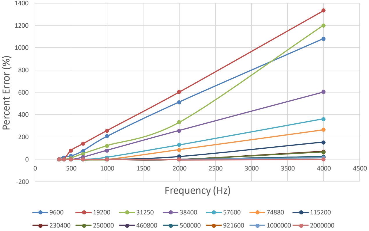
Fig 8. Relations Between Frequency and percent error.
