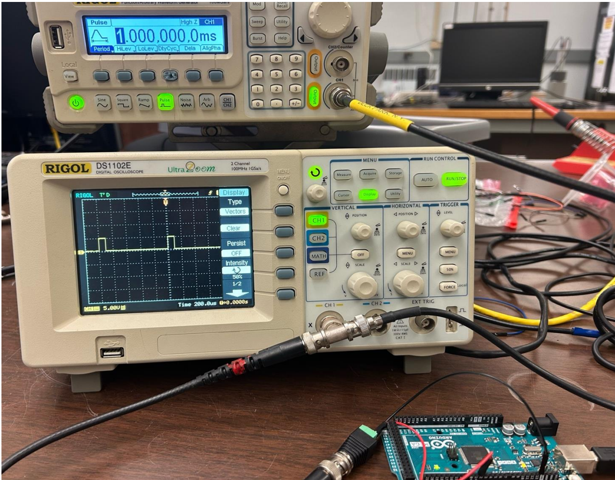
Fig 4. Whole setup
